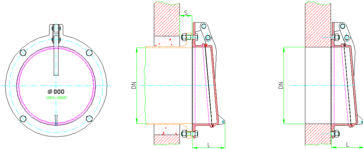
Pipe flange fixing with reduced blade thickness, suitable for local flange acc. DIN 2501 PN 10
